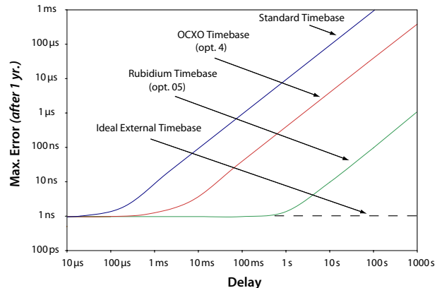
Timing error vs. programmed delay
